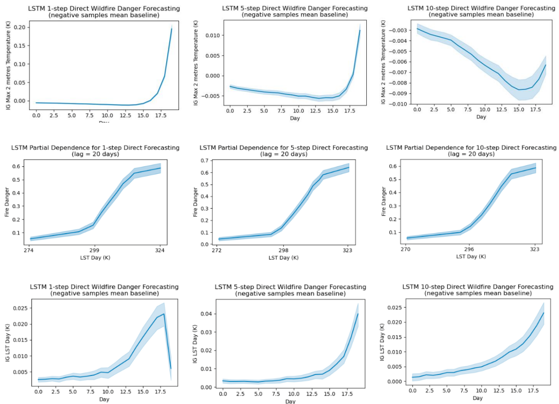
Fig. 5.5. PDP and IG plots for 1, 5 and 10-step direct forecasting using 20 days lag
