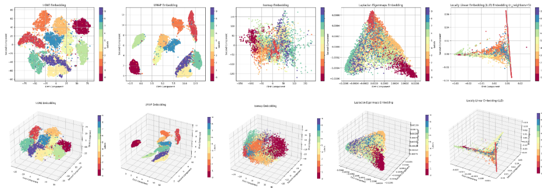
Fig. 1: MNIST plots of the main Manifold learning algorithms for dimensions 2 and 3
