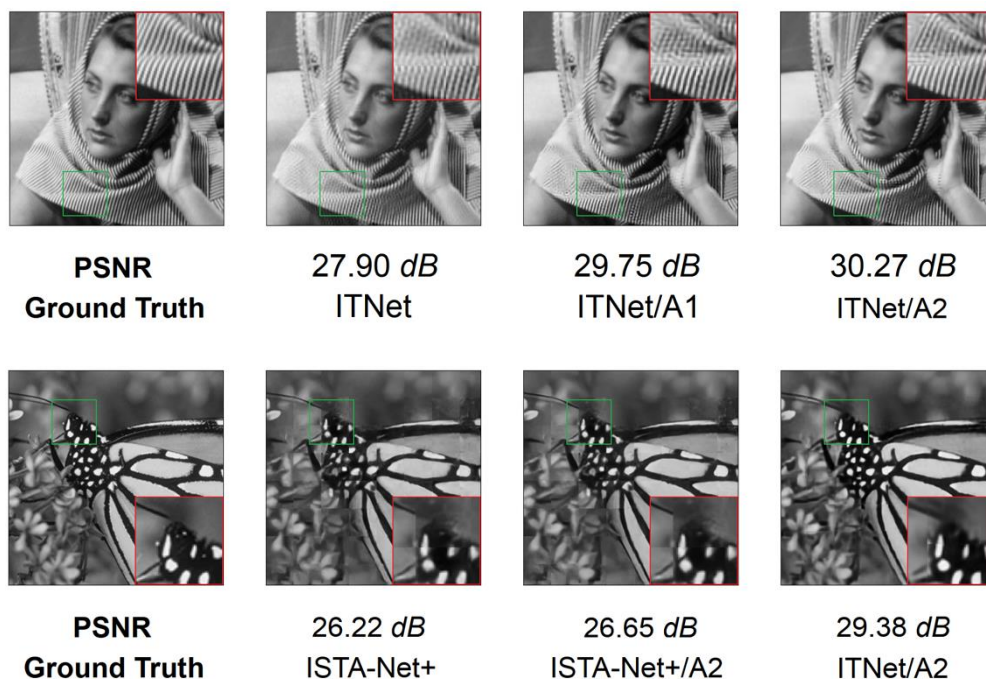
Figure 1: Visual comparison of ablation study models with the CS ratio being 10%
