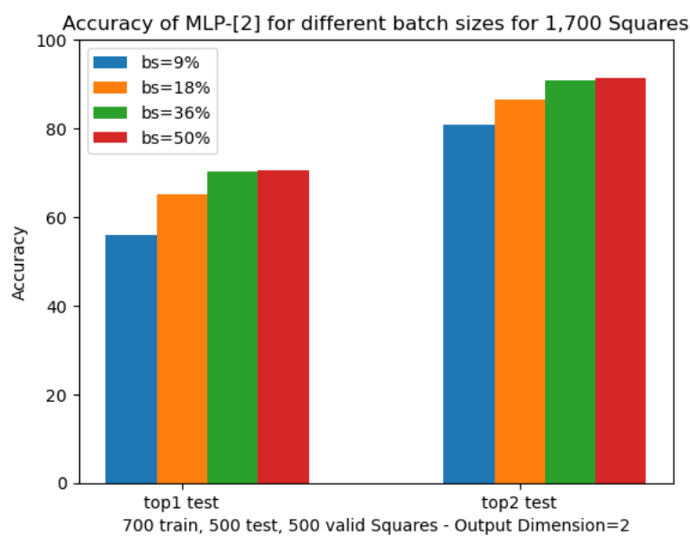
Figure 6: Batch Size for the MLP w/Isomorphy Graph
