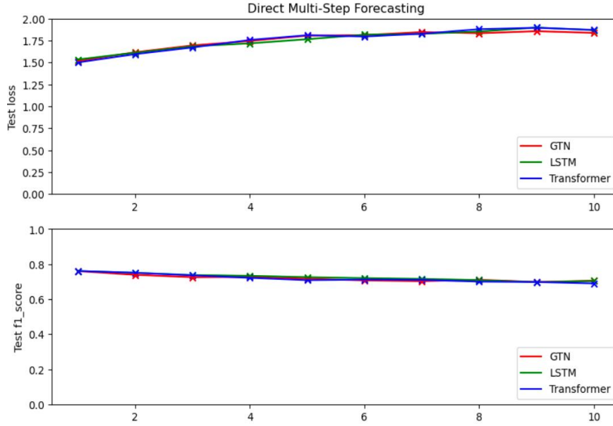
Fig. 5.2. Comparison of 1, 2, ..., 10-step Direct forecasting using the LSTM, GTN and Transformer baselines with 20 days lag based on classification metrics
