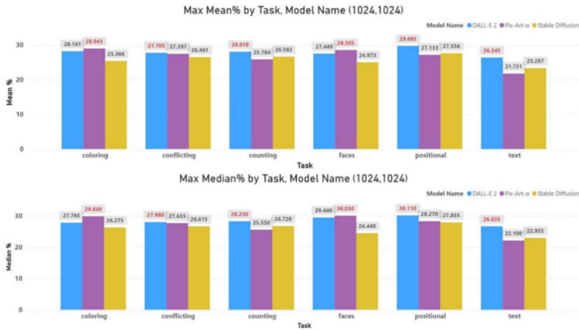
Fig. 4. Mean and Median (%) for 1024x1024 image resolution by task and model based on ViT-L/14@336px. The highest value in each cluster is highlighted in red.
