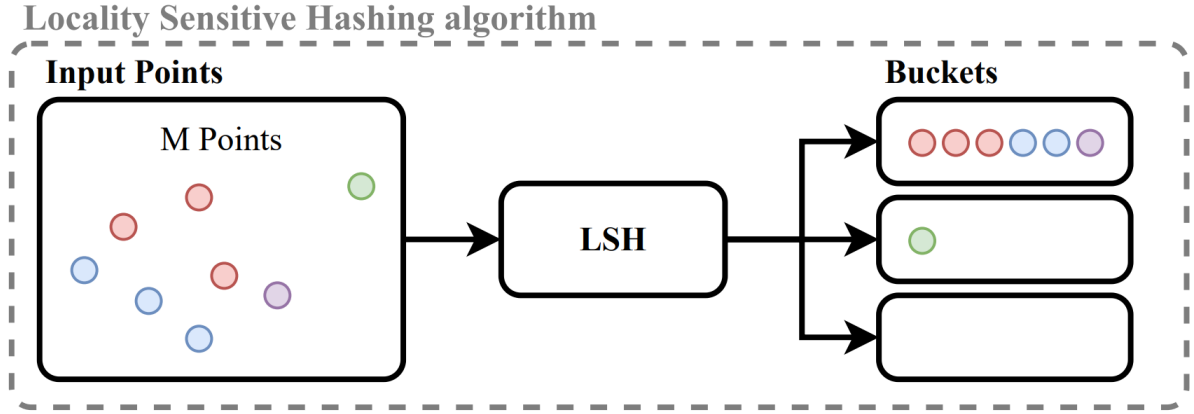
Figure 1: The diagram illustrates how the LSH algorithm works. It hashes the M input points and, after processing them, clusters them into different buckets based on their distances.
