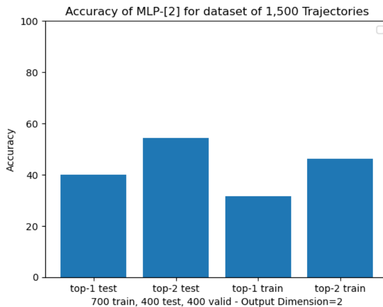
Figure 4: Accuracy of MLP w/Isomorphy for Trajectory Dataset Graph
