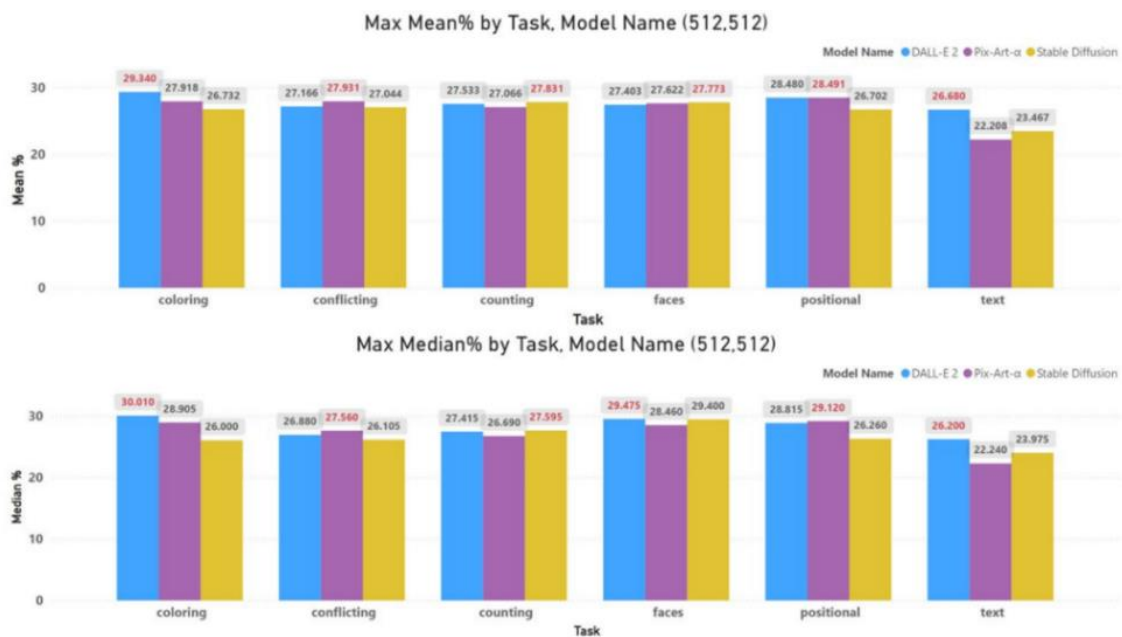
Fig. 3. Mean and Median (%) for 512x512 image resolution by task and model based on ViT-L/14@336px. The highest value in each cluster is highlighted in red.
