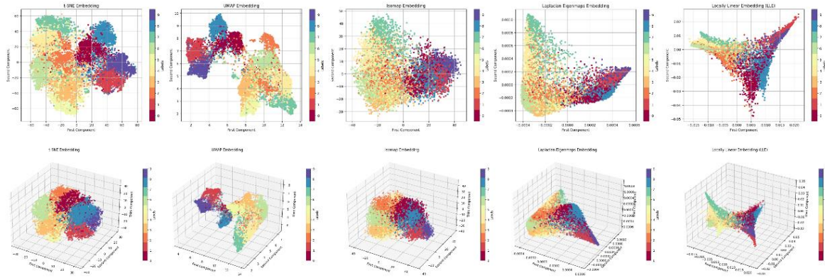
Fig. 3: Plots of methods in 2 and 3 dimensions for CIFAR10 using RESNET50
