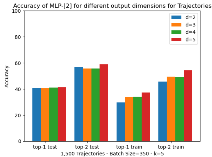
Figure 5: Output Dimension for Trajectory Dataset Graph
