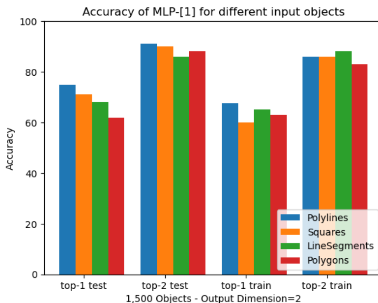
Figure 3: Accuracy of MLP w/Isometry Graph
